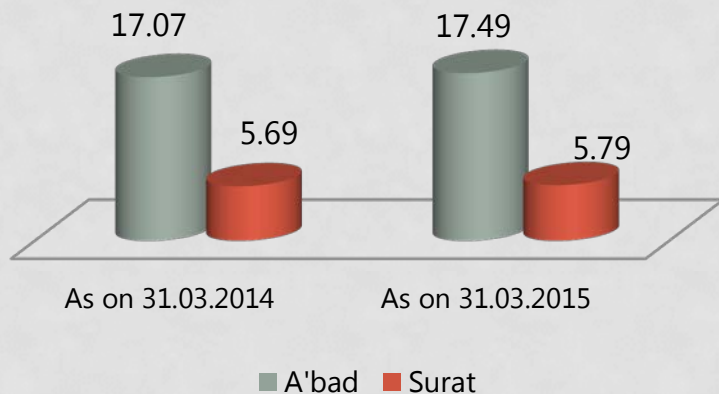
T&D loss (%)
