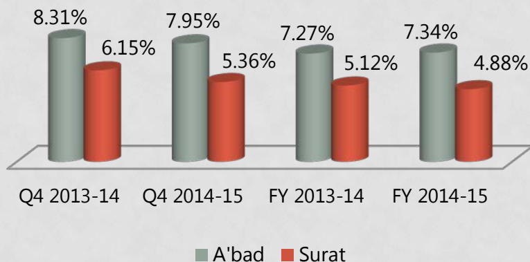
T&D loss (%)
